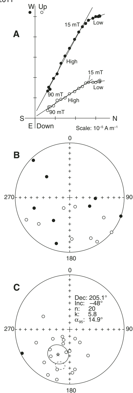
Figure 3. A: Orthogonal vector end-point diagram for a typical lapillus showing two components of magnetization. B: Equal area plot of the lapilli's high-coercivity component. C: Equal area plot of the lapilli's low-coercivity component. Solid (hollow) symbols in (B) and (C) refer to lower (upper) hemisphere projection.
