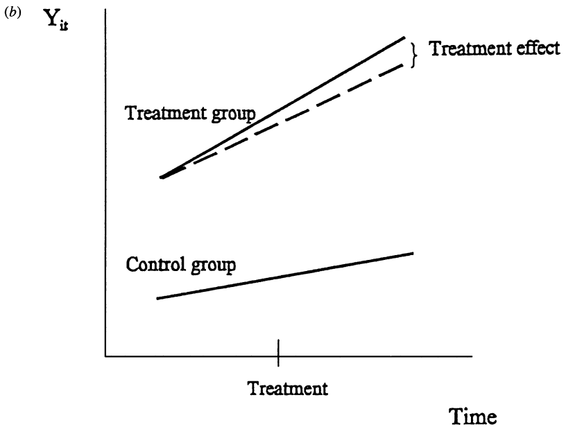
Figure 5 The true average treatment effect when unobserved heterogeneity does not differentially affect the rate of growth for both groups.
